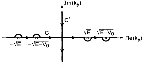
FIG. 2. Contours C and C' in the complex k_y plane.
