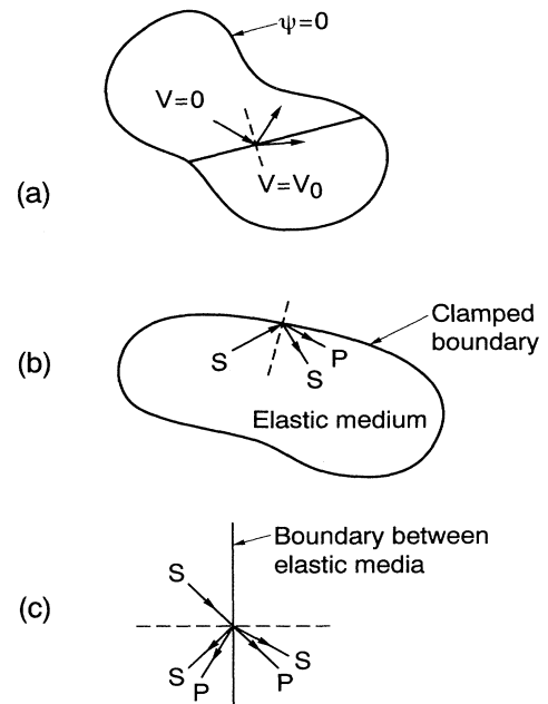
FIG. 1. Ray splitting examples. In (b) and (c) the S waves are polarized in the plane of incidence (commonly designated SV waves). For S wave motion polarized perpendicular to the plane of incidence (i.e., SH waves) there is no coupling to P waves at the boundary.
