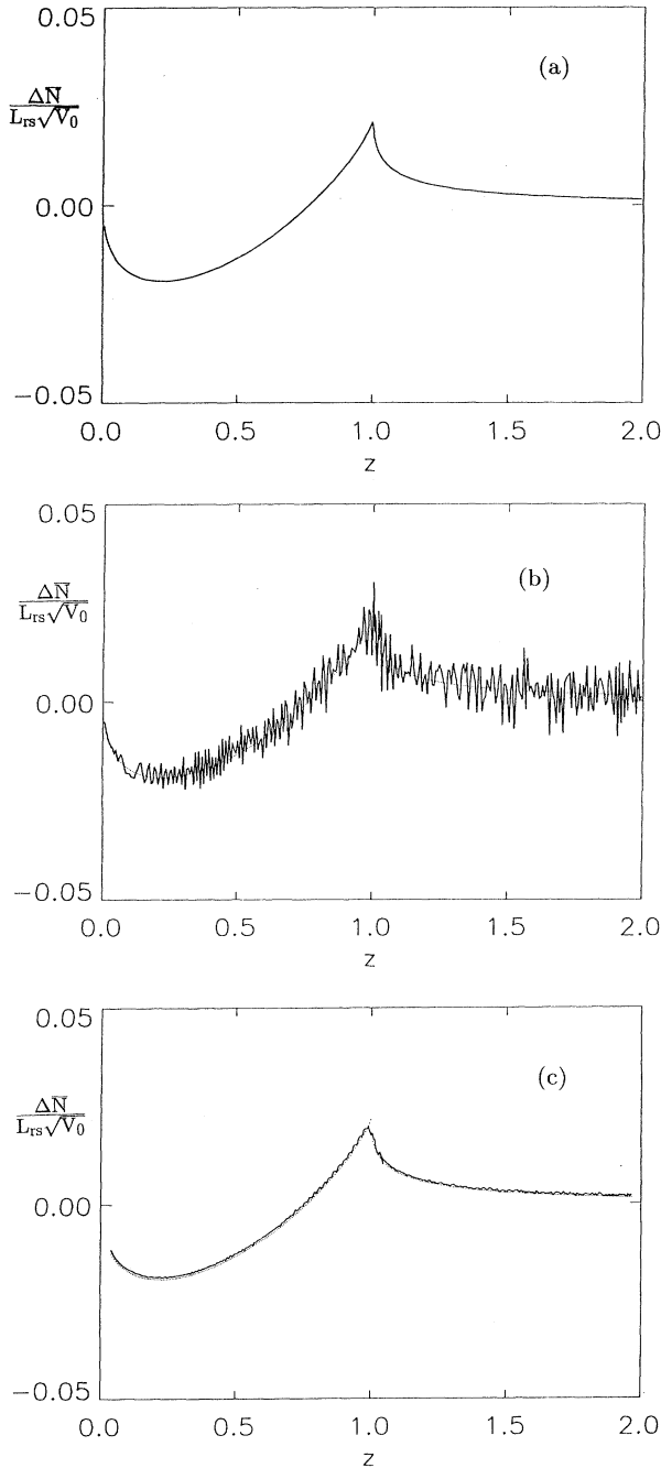
FIG. 3. \Delta\bar{N}/(L_{RS}\sqrt{V_0}) versus z .
