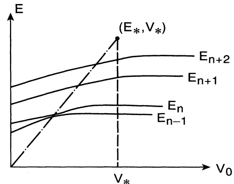
FIG. 5. Schematic illustration of E_\alpha versus V_0 .
